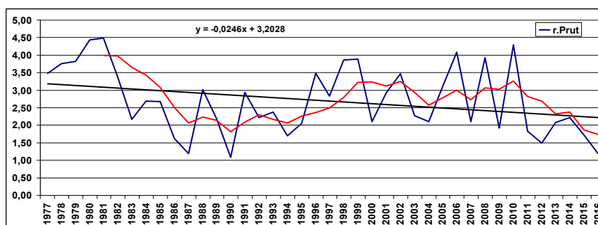
Fig. 2 b . Multiyear dynamics and change trend of total water runoff ( \text{km}^3 ) of the Prut River (1977-2016)
